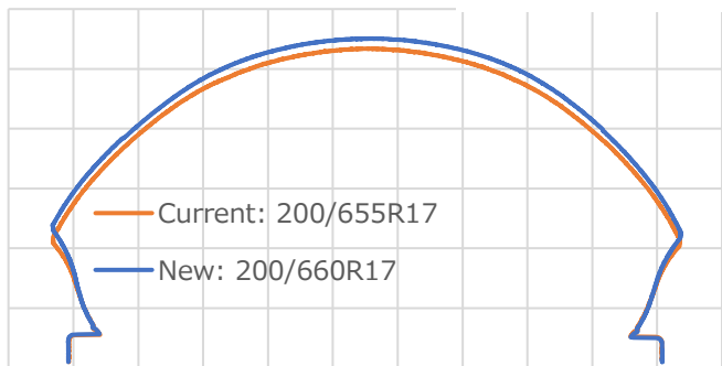
Contact Patch
