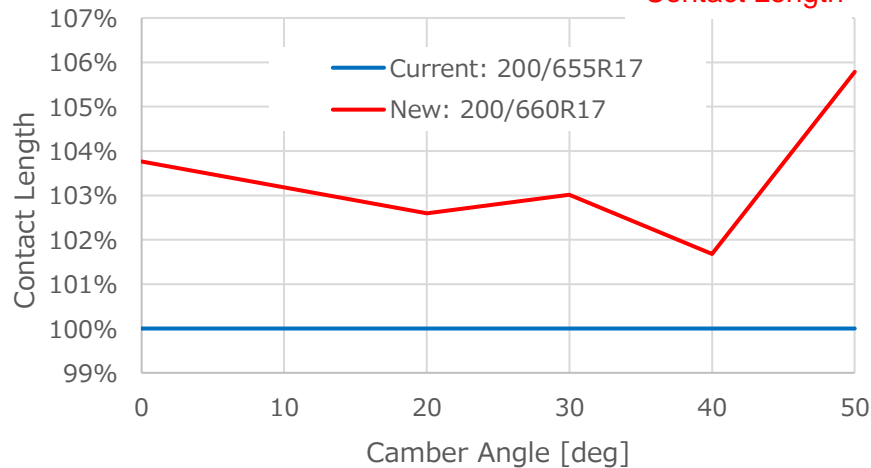
Contact Length
